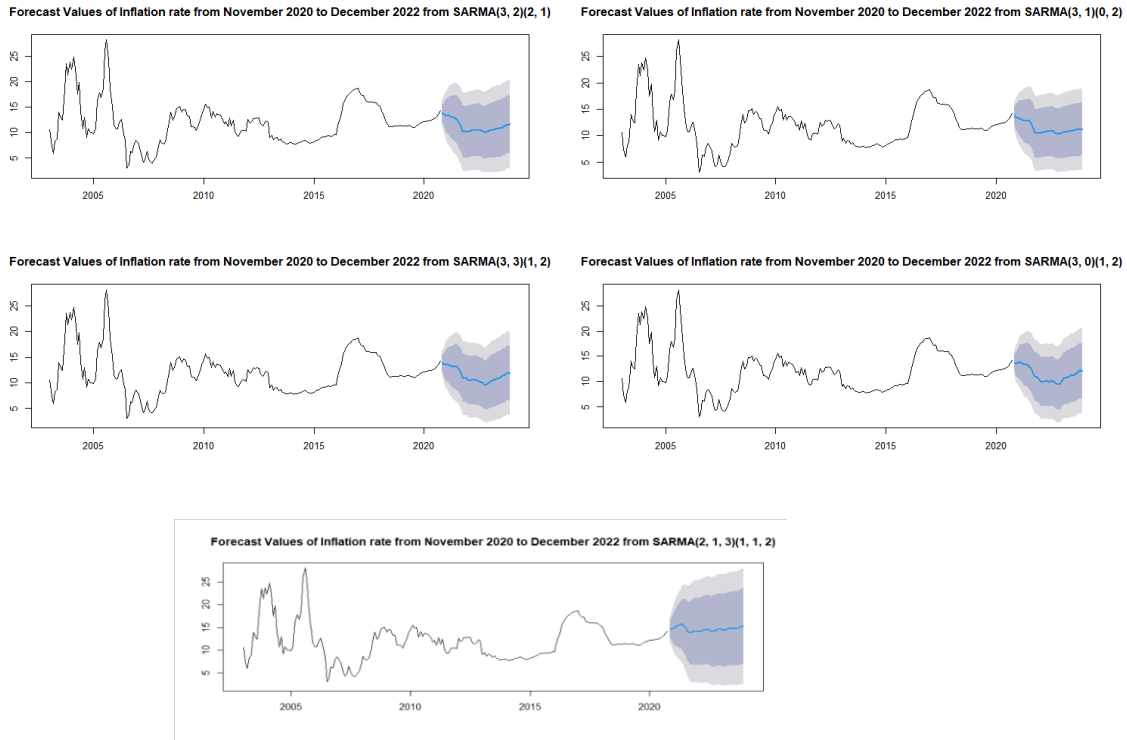
Figure 2: Plot of Forecast values of the five models
